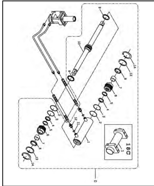
轉向油壓缸組 A303-2 STEERING CYLINDER
