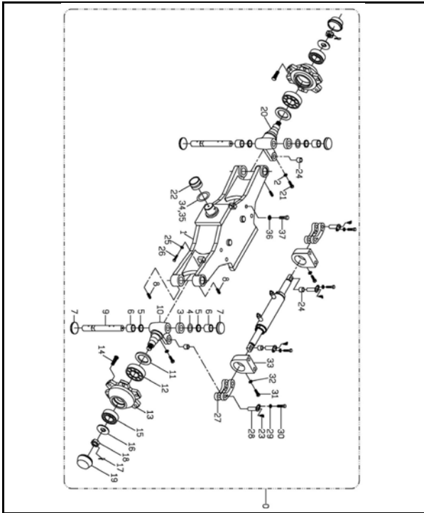
後輪樑組 A303-1 STEERING AXLE ASSY
