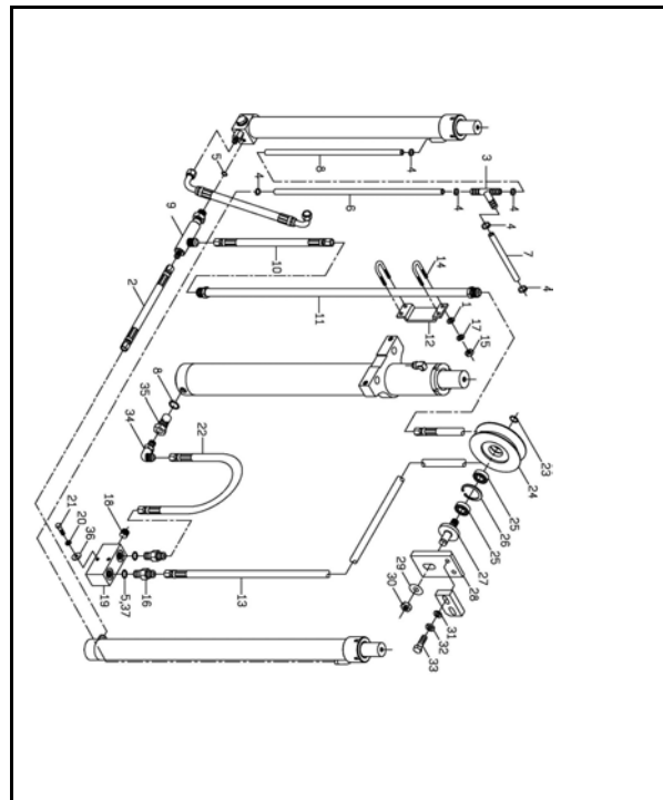
三截式升降缸配管組 A308-5B LIFT CYLINDER FITTING (THREE-STAGE)
