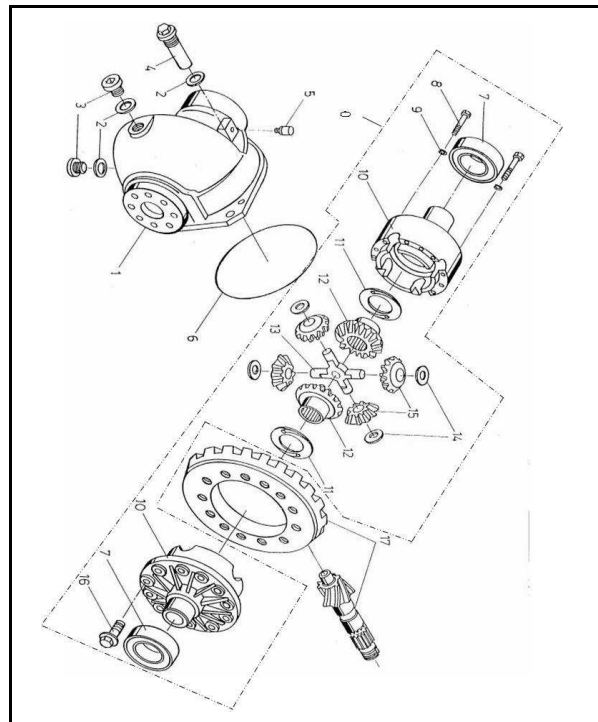
手排差速器組 A301-4 (MT) DIFFERENTIAL ASSY
