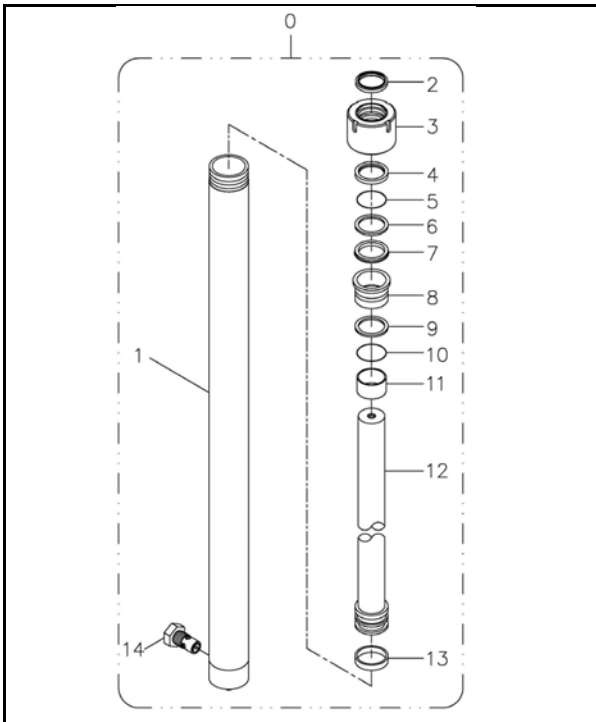
二截式貨櫃型升降缸組(左) A308-4D LIFT CYLINDER (CONTAINER FORM) (L. H.)
