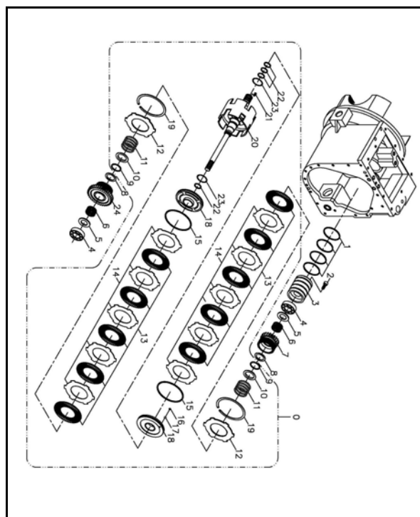
自排離合器組 A301-10 (AT) TRANSMISSION CLUTCH ASSY
