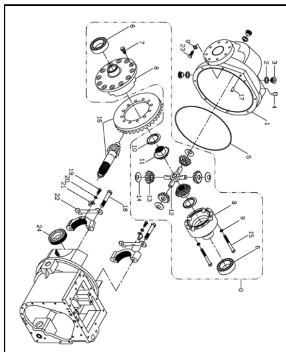
自排差速器組 A301-6 (AT) DIFFERENTIAL ASSY
