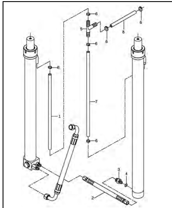
二截式升降缸配管組 A308-5 LIFT CYLINDER FITTING (TWO-STAGE)
