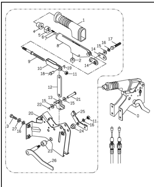
手煞車組 A306-1 PARKING BRAKE
