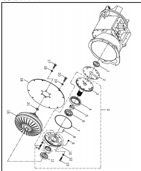
自排油泵組 A301-9 (AT) TRANSMISSION OIL PUMP
