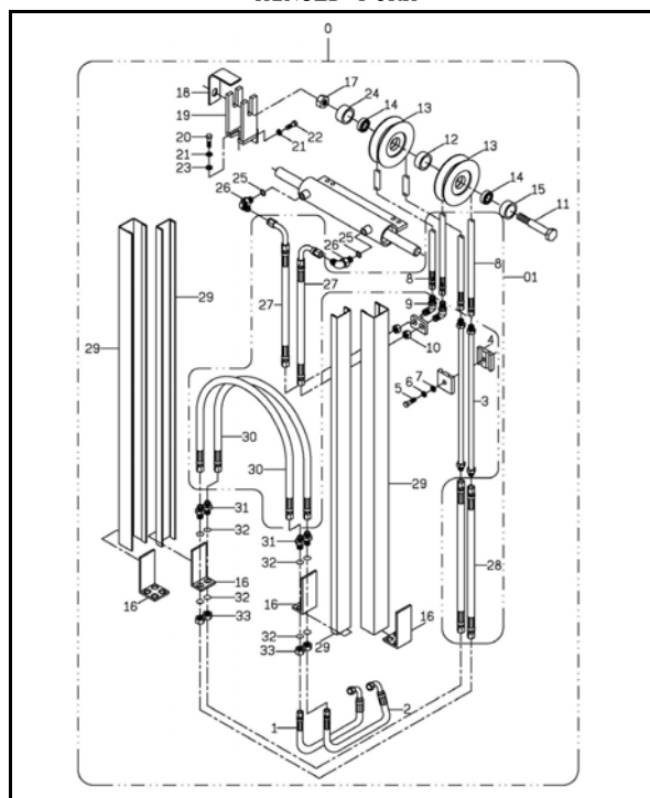
二截式貨櫃型側移配管組 A310-3A HOSE & ROLL FOR SIDE SHIFT (CONTAINER FORM)
