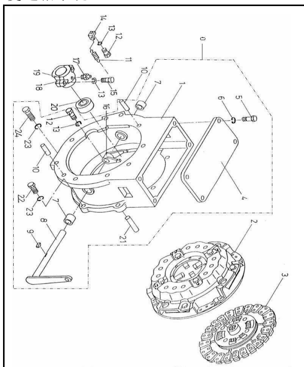
手排離合器箱組 A301-5 (MT) CLUTCH HOUSING
