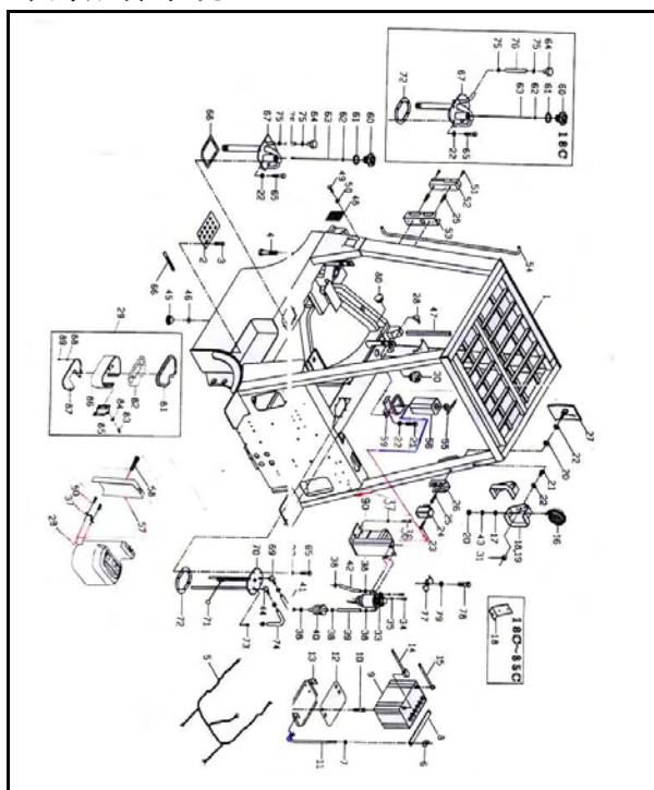
車身與配件組 A305-1 CAR BODY & FITTING
