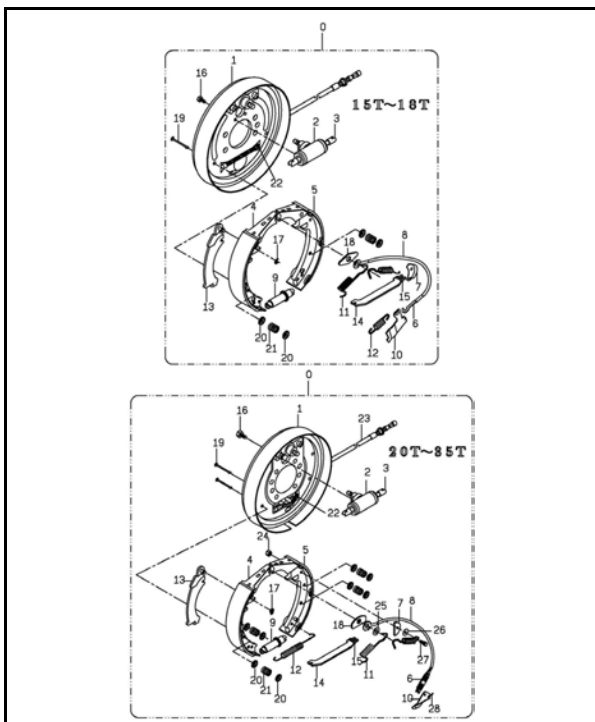
煞車襯板組 A302-2 WHEEL BRAKE ASSY
