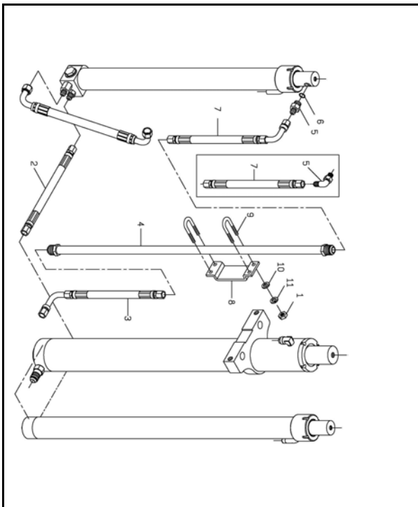
二截式貨櫃型升降缸配管組 A308-5A LIFT CYLINDER FITTING (CONTAINER FORM)
