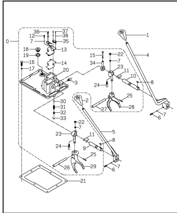
手排撥桿組 A301-2 (MT) GEARSHIFT LEVER ASSY
