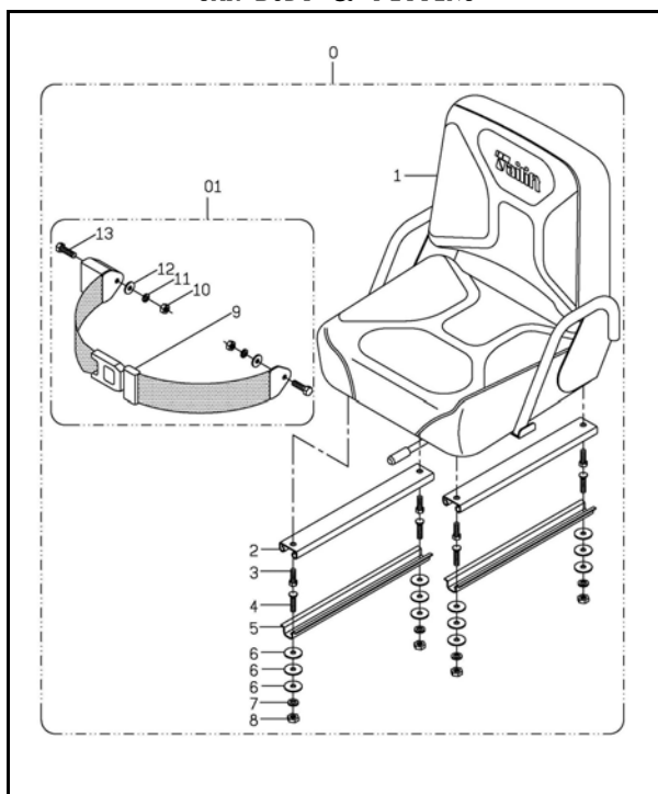
駕駛座椅組 A305-3 DRIVER SEAT
