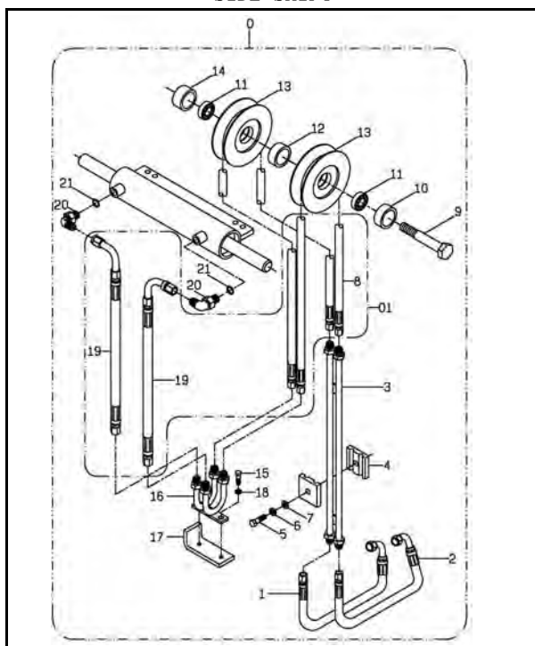
二截式側移配管組 A310-3 HOSE & ROLL FOR SIDE SHIFT (TWO-STAGE)
