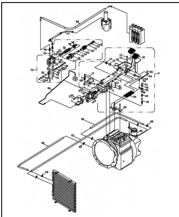
自排臥式煞車組 A306-3 (AT) HORIZONTAL-BRAKE PEDAL ASSY
