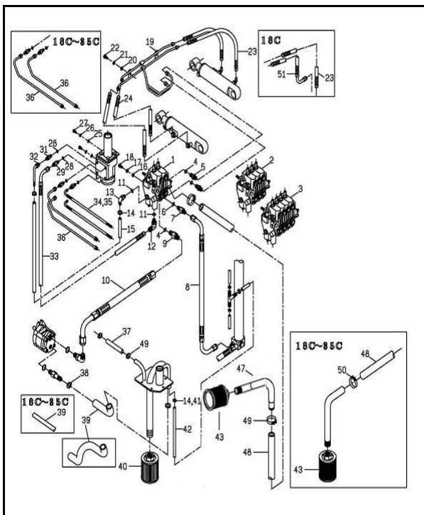
油壓管路組 A308-7 LIFT BRACKET FORK
