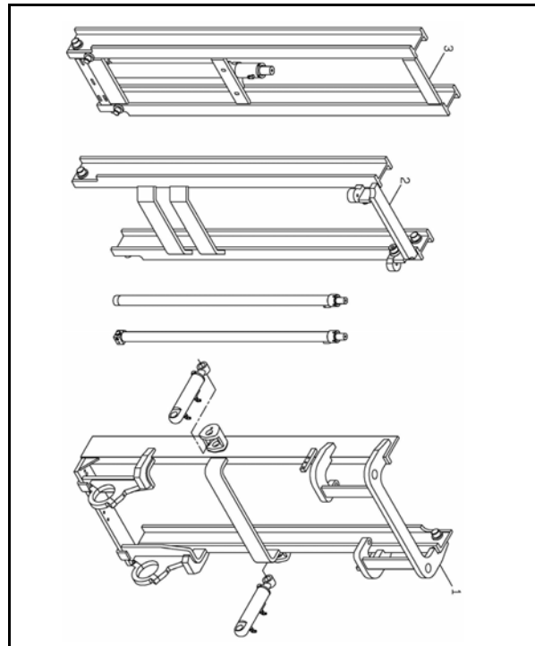
滑軌組 A308-2 MAST ASSY
