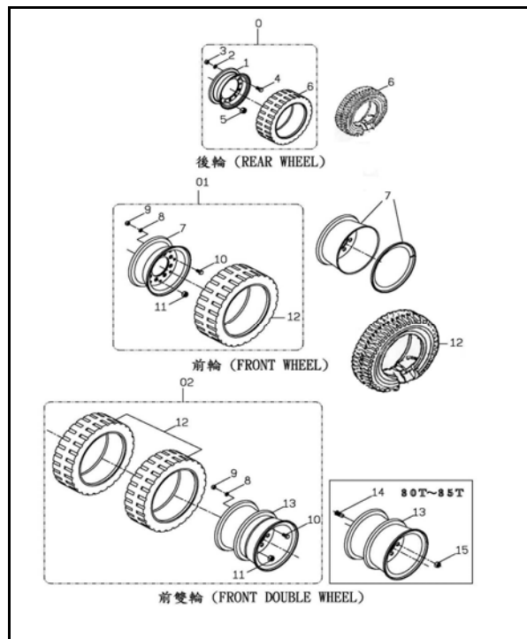
輪胎組 A302-3 TIRE ASSY
