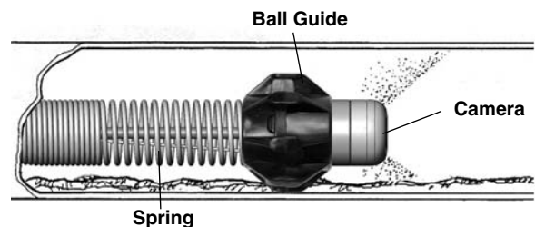
Figure 20 – Ball Guide In Use
